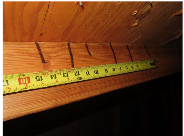
Roof deck nail spacing - Edge
